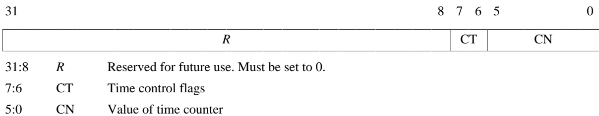
Figure 10.7. SpaceWire time code packet
